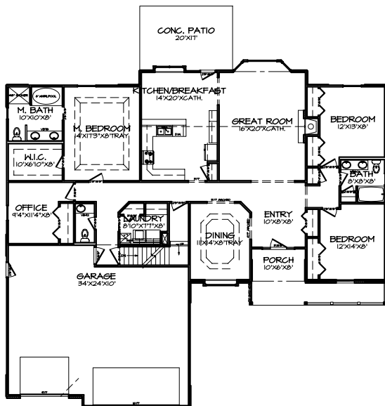
3 FIRST FLOOR PLAN A-3
