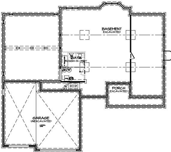
2 FOUNDATION PLAN A-2
